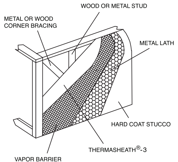
Figure 4 - Thermasheath®-3 Applied Under Hard Coat Stucco
