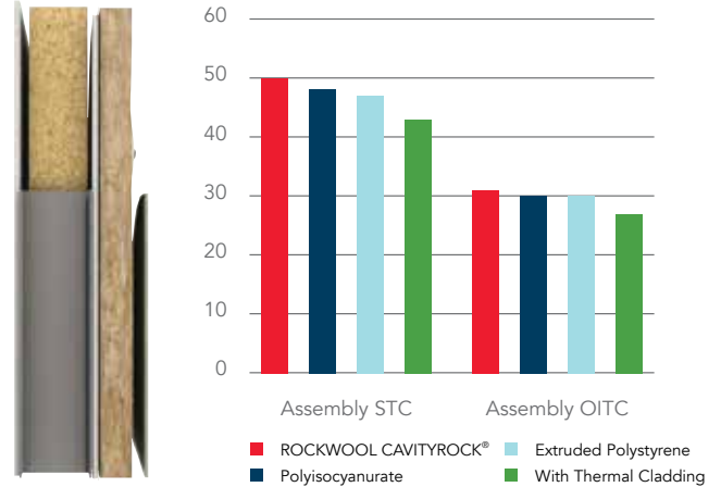
Test Wall: (Inside to Outside) 1/2" Gypsum, 6" Steel stud, ROCKWOOL Comfortbatt® insulation, 5/8" Gypsum board, Air/Vapor retarder, ROCKWOOL Cavityrock® insulation, 3/8" Cement board cladding.
